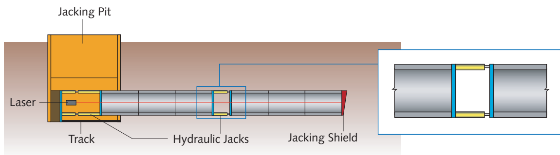
Typical Jacking Arrangement
